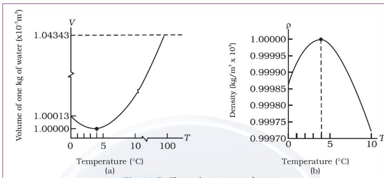
Fig. 11.7 Thermal expansion of water
